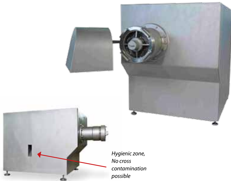
Large in-feed hopper for both fresh and frozen meat raw materials
