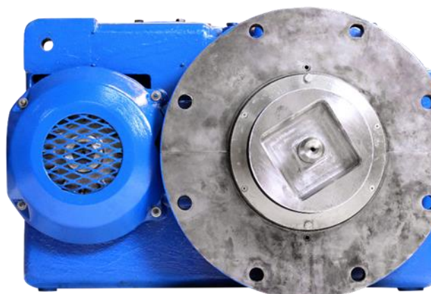
David Brown gear box after refurbishment
