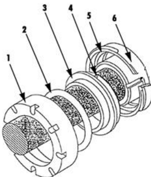
Mixing Wing Seal Assembly
